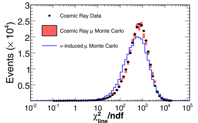
FIG. 8 (color online). Comparison of the \chi_{\text{line}}^2/\text{ndf} distributions for stopping muons in the cosmic ray data (points), in the cosmic ray Monte Carlo simulation (boxes), and in the neutrino-induced Monte Carlo simulation (line). The number of events in each bin for the cosmic ray Monte Carlo simulation is shown by the location of the center of the box for the bin, and the vertical extent of the box indicates the statistical uncertainty in the bin.
