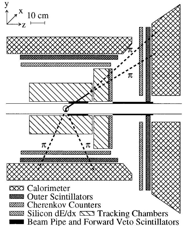
FIG. 1. Schematic view of the Jetset detector with a K_S K_S event superimposed.
