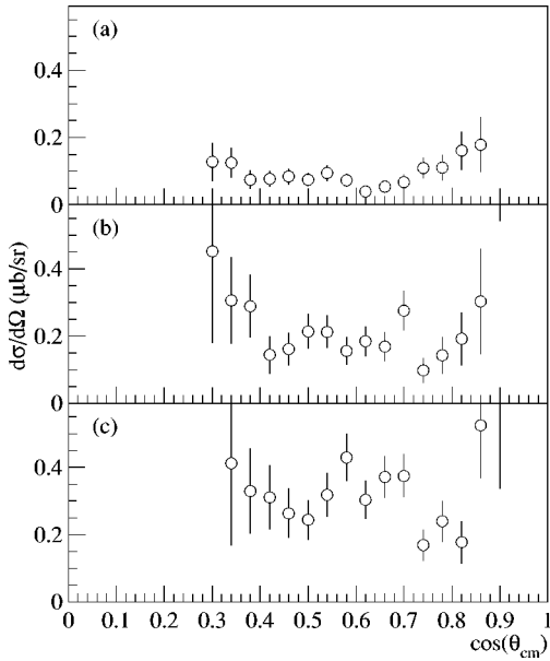
FIG. 6. Differential cross section results for three energy groupings of the reaction \bar{p}p \rightarrow K_S K_S . The 1.2-, 1.3-, 1.4-, and 1.5-GeV/ c data are shown in (a), the fine-scan (1.39–1.48)-GeV/ c data are shown in (b), and the 1.6-, 1.7-, 1.8-, and 1.9-GeV/ c data are shown in (c).
