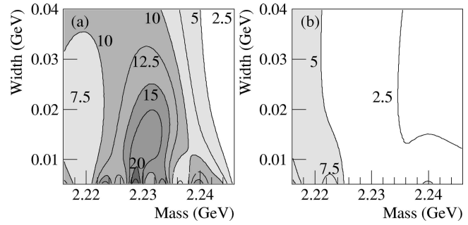
FIG. 7. Contours of the upper limit on the double branching ratio B(\xi \rightarrow \bar{p}p) \times B(\xi \rightarrow K_S K_S) as a function of resonance mass and width for a J=2 resonance. The contours represent steps of 2.5 \times 10^{-5} and the shading changes in steps of 5 \times 10^{-5} . In (a) only the data from this work are considered. In (b) our data are combined with the data from PS185 [8] and the same procedure is repeated.
