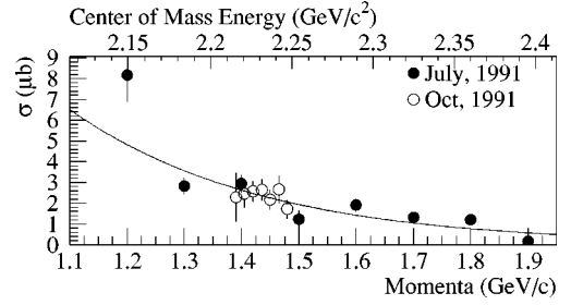
FIG. 5. Total cross section for the reaction \bar{p}p \rightarrow K_S K_S . The solid curve is a fit following the form A p^* \times e^{-B p^*} , excluding the 1.2 GeV/c point. The fine-scan data have been adjusted to match the scale of the coarse-scan data by means of a multiplicative factor.
