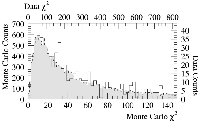
FIG. 2. \chi^2 distributions for data (unshaded, solid line) and Monte Carlo events (shaded, dashed line). The lower and left scales are for the Monte Carlo events and the upper and right scales are for data.
