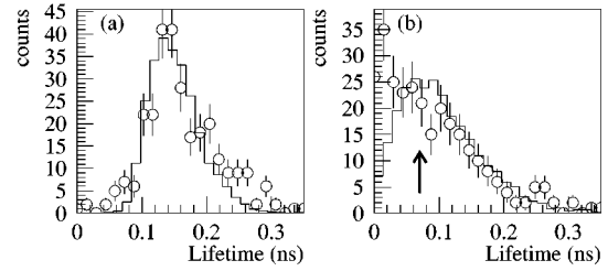
FIG. 4. Lifetime distributions for the fine-scan data (points) and Monte Carlo events (histogram) for (a) forward and (b) barrel vertices. The arrow indicates where the “tail” began for purposes of the fit.
