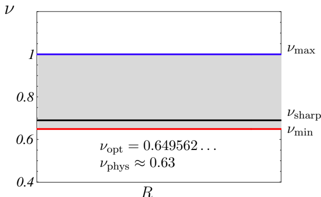
Figure 1: Critical exponent \nu for various R , N = 1 . The shaded region contains about 10^3 data points for various classes of cutoffs. We have indicated the sharp cutoff result (black line), the numerical result \nu_{\max} at the upper boundary (blue line) and at the lower boundary \nu_{\min} = \nu_{\text{opt}} (red line). The latter coincides with the result from the optimised ERG flow (3.6) and the Polchinski flow (3.7). The physical value is also indicated (see text).
