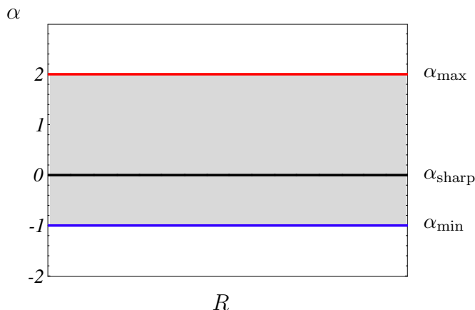
Figure 2: Large-field behaviour of wilsonian flows close to a critical point, d = 3 . The shaded region indicates the range of values for \alpha(R) for various R . The sharp cutoff (black line) marks the boundary between flows with significant ( \alpha < 0 ) and insignificant ( \alpha > 0 ) contributions at large fields. Callan-Symanzik type flows and the Polchinski flow have \alpha = \alpha_{\min} (blue line), generic ERG flows have \alpha = \alpha_{\max} (red line). Flows with an increased locality structure lead to improved results (see text).
