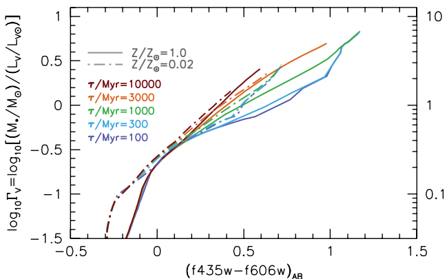
Figure 2. Evolutionary tracks ( t = 0 \rightarrow t_{\text{uni}}(z = 0) ) of stellar populations in the rest-frame (f435w - f606w)_{\text{AB}} - V -band mass-to-light ratio plane, created assuming a Salpeter (1955) IMF, utilizing the PEGASE.2 SPS model and assuming several exponentially declining star formation histories ( \psi \propto e^{-t/\tau} with \tau/\text{Gyr} \in \{0.1, 0.3, 1.0, 3.0, 10.0\} ) and two metallicities ( Z/Z_{\odot} = 1 and Z/Z_{\odot} = 0.02 ) as indicated by the key.
