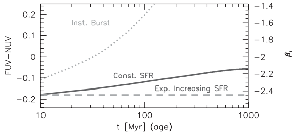
Figure 2. The effect of the duration and form of previous SF on the UVC colour. The three lines show the evolution of the UVC colour (left) and slope (right) of a stellar population-forming stars at a constant rate (solid line), an exponentially increasing rate (dashed line) and as an instantaneous burst (dotted line).
