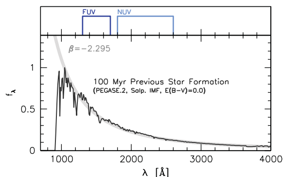
Figure 1. The synthetic UV spectrum of a star-forming galaxy (100 Myr of previous continuous SF, Salpeter IMF, Z = Z_{\odot} ) produced with the PEGASE.2 population synthesis model (black line). The heavy grey line is a pure power law f_{\lambda} \propto \lambda^{\beta} assuming the value of \beta inferred from the FUV–NUV colour (transmission functions shown in the upper panel).
