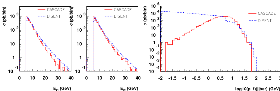
Figure 8: Comparison of the k_{\perp} -shower CASCADE with the NLO di-jet calculation DISSENT: (left) distribution in single-jet transverse energy; (right) distribution in the di-jet transverse energy.
