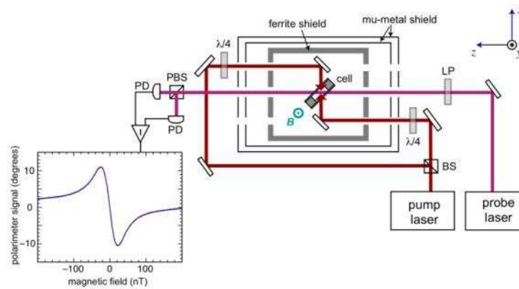
Fig. 2. Experimental setup. BS: beamsplitter, LP: linear polarizer, \lambda/4 : quarter wave plate, PBS: polarizing beamsplitter, PD: silicon PIN photodiode.
