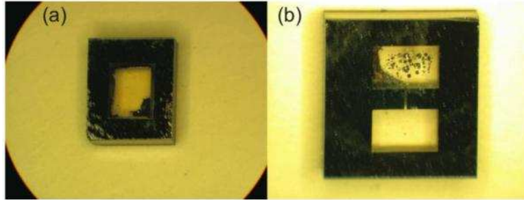
Fig. 1. Microfabricated vapor cells: (a) 3 mm x 2 mm x 1 mm single-chambered cell, (b) dual-chambered cell with two 3 mm x 2 mm x 1 mm cavities connected by a 1 mm x 0.1 mm passage.
