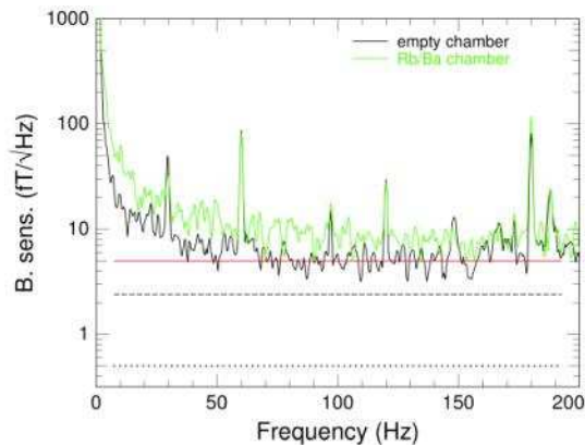
Fig. 3. Magnetic field sensitivity versus frequency in a dual-chambered microfabricated vapor cell. The red line indicates a sensitivity of 5 \text{ fT/Hz}^{1/2} . The dashed line shows the estimated sensitivity limit due to photon shot noise, and the dotted line shows an estimate of the atom (spin-projection) noise based on App. A in Ref. [19].
