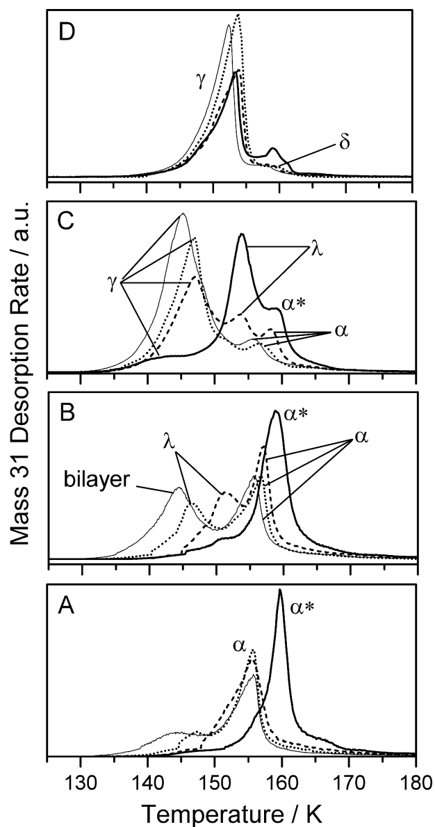
Fig. 3 Comparison of TPD spectra for C_2H_5OH adsorbed on 2 L (dotted line), 10 L (dashed line) and 50 L (thick solid line) H_2O films. C_2H_5OH desorption from a bare HOPG surface adsorbed at 98 K is also shown for comparison (thin solid line). C_2H_5OH exposures are (A) 5 L, (B) 10 L, (C) 50 L and (D) 300 L, showing the changes in the C_2H_5OH desorption features as a function of H_2O exposure.
