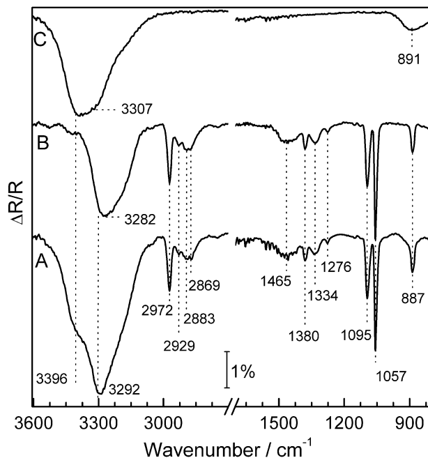
Fig. 7 Trace A shows the RAIR spectrum for a 300 L exposure of C_2H_5OH deposited on top of a 50 L H_2O film adsorbed on HOPG at 98 K. Traces B and C show RAIR spectra for pure C_2H_5OH (300 L) and pure H_2O (50 L), respectively, adsorbed on HOPG at 98 K. The region between 2700\text{ cm}^{-1} and 1700\text{ cm}^{-1} , which contains no infrared bands, has been omitted for clarity.
