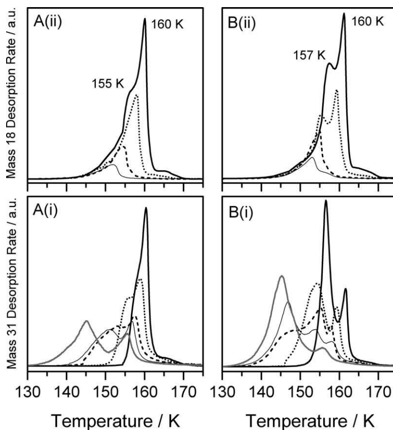
Fig. 5 TPD spectra following increasing exposures of H 2 O deposited onto pre-existing C 2 H 5 OH films adsorbed on HOPG at 98 K. Fig. (A) shows (i) C 2 H 5 OH and (ii) H 2 O desorption traces from a 15 L C 2 H 5 OH film. (B) shows the corresponding (i) C 2 H 5 OH and (ii) H 2 O TPD arising from a 50 L C 2 H 5 OH film. In each case the H 2 O exposures were 10 (thin solid lines), 20 (dashed lines), 50 (dotted lines) and 100 L (thick solid lines). The corresponding pure C 2 H 5 OH TPD traces (grey solid lines) are included for comparison.
