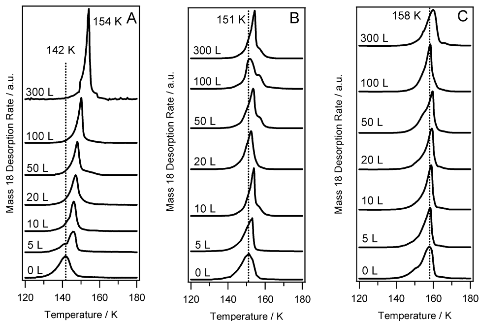
Fig. 1 TPD spectra showing the desorption of H 2 O from layered binary C 2 H 5 OH/H 2 O ices for exposures of (A) 2 L, (B) 10 L and (C) 50 L H 2 O grown on HOPG at 98 K. C 2 H 5 OH exposures deposited onto the H 2 O films are shown in the figure. TPD traces for pure H 2 O ices with no C 2 H 5 OH overlayer are also shown.
