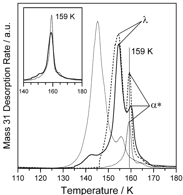
Fig. 6 TPD spectra comparing the desorption of 50 L C_2H_5OH from different ice configurations: C_2H_5OH adsorbed on top of a 50 L H_2O film (thick solid line), C_2H_5OH dosed underneath a 50 L H_2O film (dashed line) and C_2H_5OH desorption from a bare HOPG surface (thin solid line). The dotted line shows C_2H_5OH desorption from a co-deposited C_2H_5OH:H_2O mixture (1:5 ratio) and corresponds to an equivalent exposure of 10 L of pure C_2H_5OH . The inset compares the TPD spectrum from a co-deposited C_2H_5OH:H_2O mixture (dotted line) shown in the main figure to C_2H_5OH desorption from 10 L C_2H_5OH deposited on a 50 L H_2O film (solid line). In each case the substrate temperature was 98 K.
