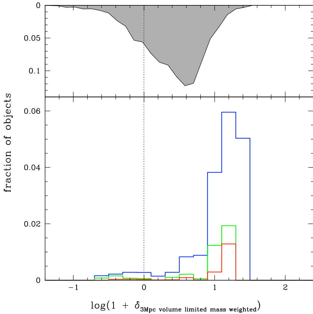
Fig. 4: Lower panel: The fraction of galaxies in the 10k sample that would be associated as a close kinematic pair if an additional galaxy is randomly inserted into the density field. Close pairs with projected separations of dr < 100 h^{-1} \text{kpc} are in blue, dr < 50 h^{-1} \text{kpc} in green, and dr < 30 h^{-1} \text{kpc} in red. Top panel: the distribution of over-densities of objects in the 10k sample.
