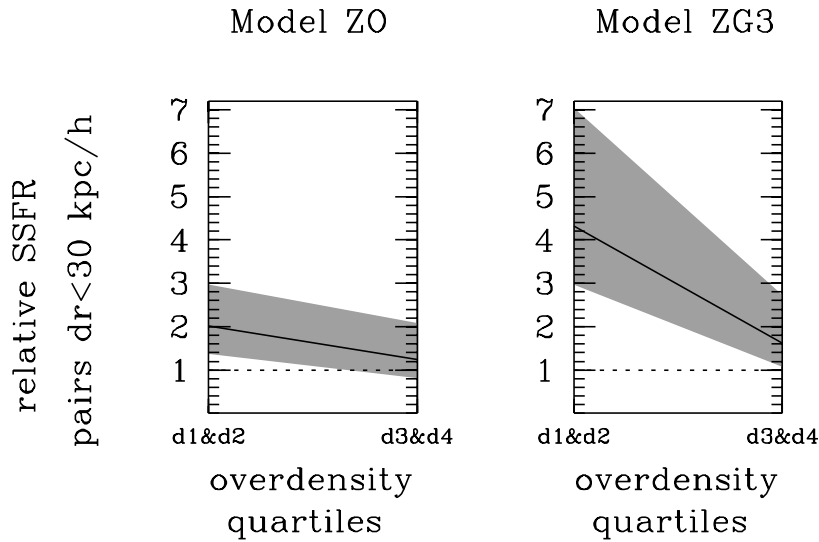
Fig. 17: Relative average sSFR in the close kinematic pair galaxies with projected distances less than 30 h^{-1}kpc in respect to the sSFR derived for 2 different models in our Monte Carlo simulations as a function of environment. Galaxies in lower than median over-density quartiles D1 & D2 show much stronger enhancement in sSFR than the galaxies residing in higher than median over-density quartiles D3 & D4. The two models are: “ZO” – redshift distribution and over-densities as in the pair galaxies; “ZG3” – redshift distribution as in the pair galaxies and galaxies are in a group catalog with an observed richness of 3 or higher.
