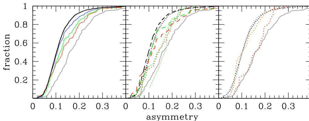
Fig. 16: Cumulative distributions of asymmetries: on all panels the grey solid line represent the distribution of asymmetries for 115 visually selected merger candidates in the COSMOS at z=0.7-0.8 (Kampczyk et al. 2007). The left panel presents distributions for galaxies in the underlying sample (black), the close kinematic pair galaxies with projected separations less than 100 h^{-1} \text{kpc} (blue), less than 50 h^{-1} \text{kpc} (green) and less than 30 h^{-1} \text{kpc} (red). The central panel shows distributions with the same color scheme as before, but the distributions are divided according to the environments – dotted lines for the galaxies that reside in the lower than median over-density, dashed – above the median over-density. Dotted light green–light red line on the right side of the grey solid one represents the data for the lowest quartile (D1) of the over-density distribution for the close pairs with less than 50 h^{-1} \text{kpc} and less than 30 h^{-1} \text{kpc} (both samples coincide in this quartile). The right panel presents the result of splitting the underlying sample with lower than median over-densities into two redshift subsamples of an equal size – the high redshift one (black dotted line) and the low redshift one (grey dotted line). The close kinematic pair galaxies with projected separations less than 30 h^{-1} \text{kpc} were split around the same redshift into the high redshift bin (red dotted line) and the low redshift one (orange dotted line).
