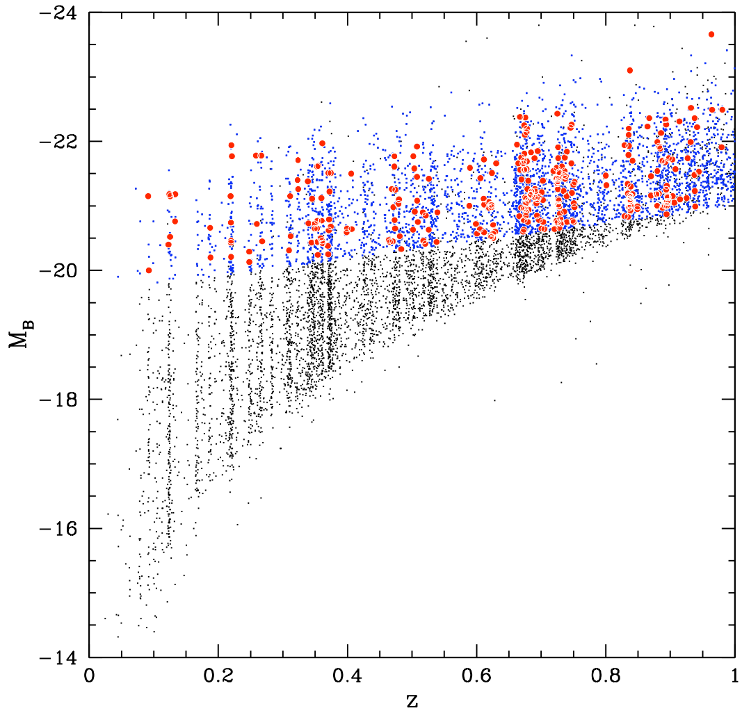
Fig. 3: The rest frame B-band absolute magnitude as a function of redshift for the zCOSMOS 10k sample. The blue points represent galaxies with secure redshifts above the absolute magnitude cut ( M_B < -19.64 - 1.36 z ) among which pair galaxies are highlighted with red dots.
