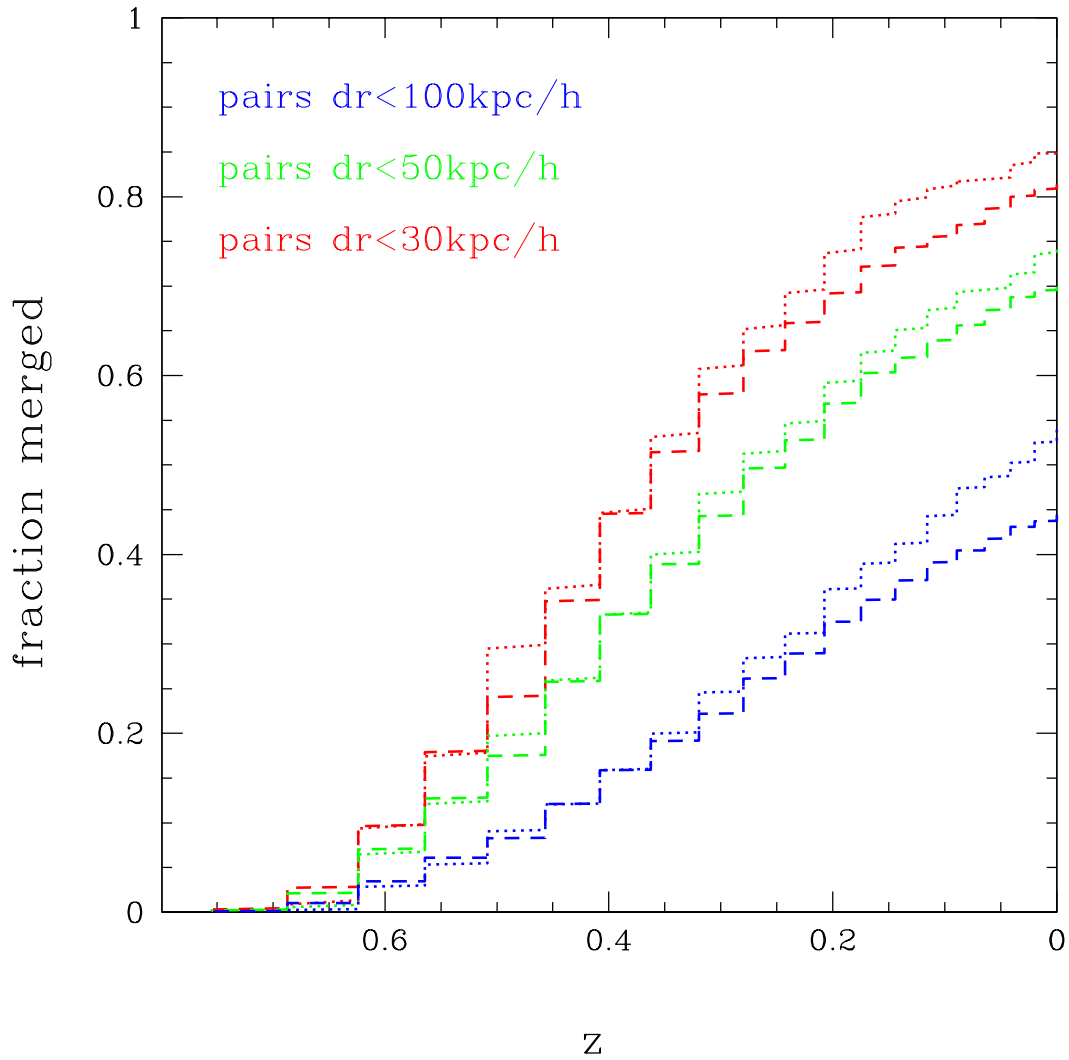
Fig. 6: The cumulative redshift distribution of merger events in close kinematic pairs of galaxies selected in the redshift range 0.6 < z < 0.8 from the Kitzbichler 2006 mocks of the Millennium simulation. Galaxy pairs were chosen with the same absolute magnitude cut and major merger criterion as in our observed sample: dr < 100 h^{-1}kpc in blue, dr < 50 h^{-1}kpc in green, and dr < 30 h^{-1}kpc in red. Dashed lines indicate the distributions for pairs residing in environments denser than the median of an underlying density distribution, dotted – residing in a lower than the median. The fraction of galaxies that merged by z = 0 is indicated by the values at z = 0 .
