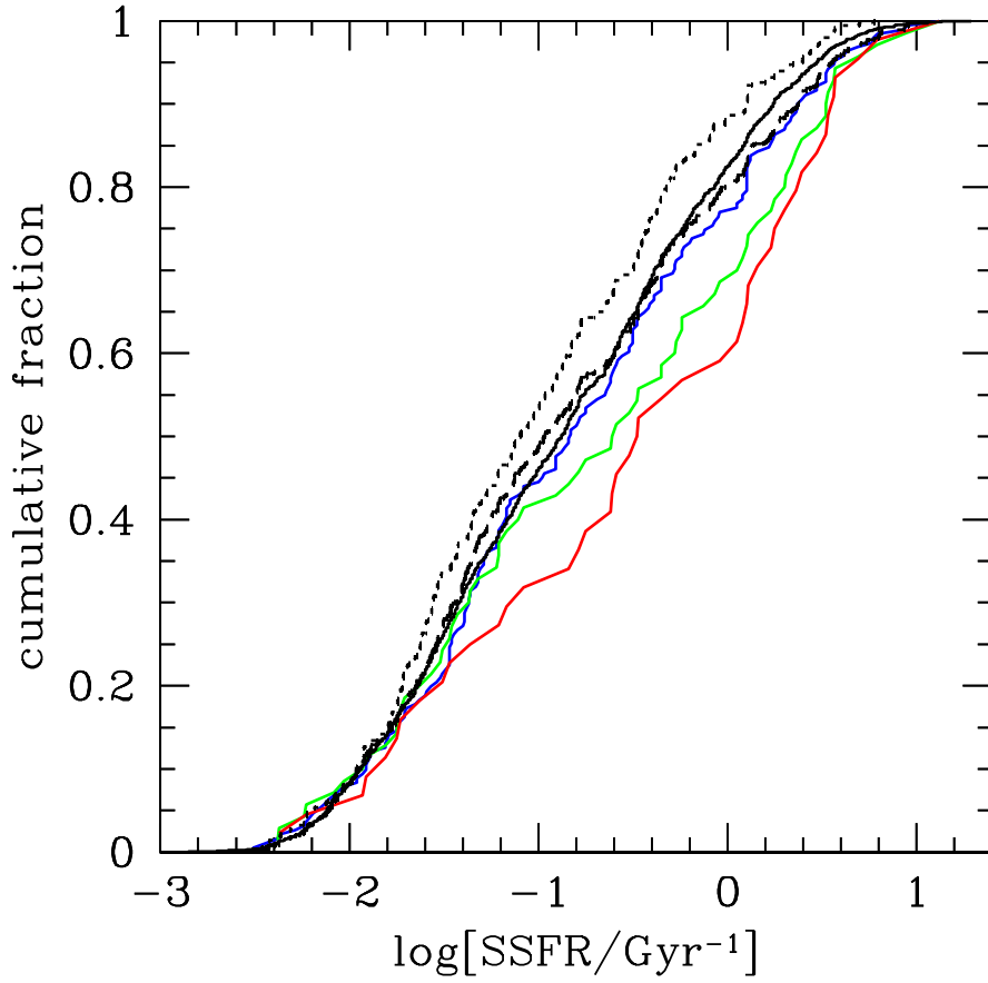
Fig. 13: Cumulative distribution of sSFR based on [OII] 3727 measurements for Monte Carlo comparison samples in black “ZO” – redshift distribution and overdensities as in the pair galaxies (solid line); “ZG”- redshift distribution as in the pair galaxies and galaxies are in a group catalog (dashed line); “ZG3” – redshift distribution as in the pair galaxies and galaxies are in a group catalog with an observed richness of 3 or higher (dotted line). The sSFR of galaxies in pairs is indicated with colors: blue – with dr < 100 h^{-1}kpc , green – with dr < 50 h^{-1}kpc , red – with dr < 30 h^{-1}kpc .
