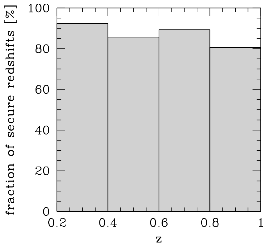
Fig. 1: Redshift completeness of the zCOSMOS 10k subsample with secure redshifts in a volume limited sample defined with an absolute magnitude cut M_B < -19.64 - 1.36z .
