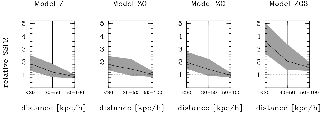
Fig. 14: Relative average sSFR in the close kinematic pair galaxies with respect to the sSFR derived for 4 different models in Monte Carlo simulations as a function of projected separations in 3 bins: less than 30 h^{-1}kpc , 30 - 50 h^{-1}kpc and 50 - 100 h^{-1}kpc . Filled areas show the derived 68% confidence interval. The four models indicated on the plots are: “Z” – galaxies drawn randomly from all galaxy sample to follow redshift distribution as in pair galaxies; “ZO” – redshift distribution and overdensities as in the pair galaxies; “ZG”- redshift distribution as in the pair galaxies and galaxies are in a group catalog; “ZG3” – redshift distribution as in the pair galaxies and galaxies are in a group catalog with an observed richness of 3 or higher.
