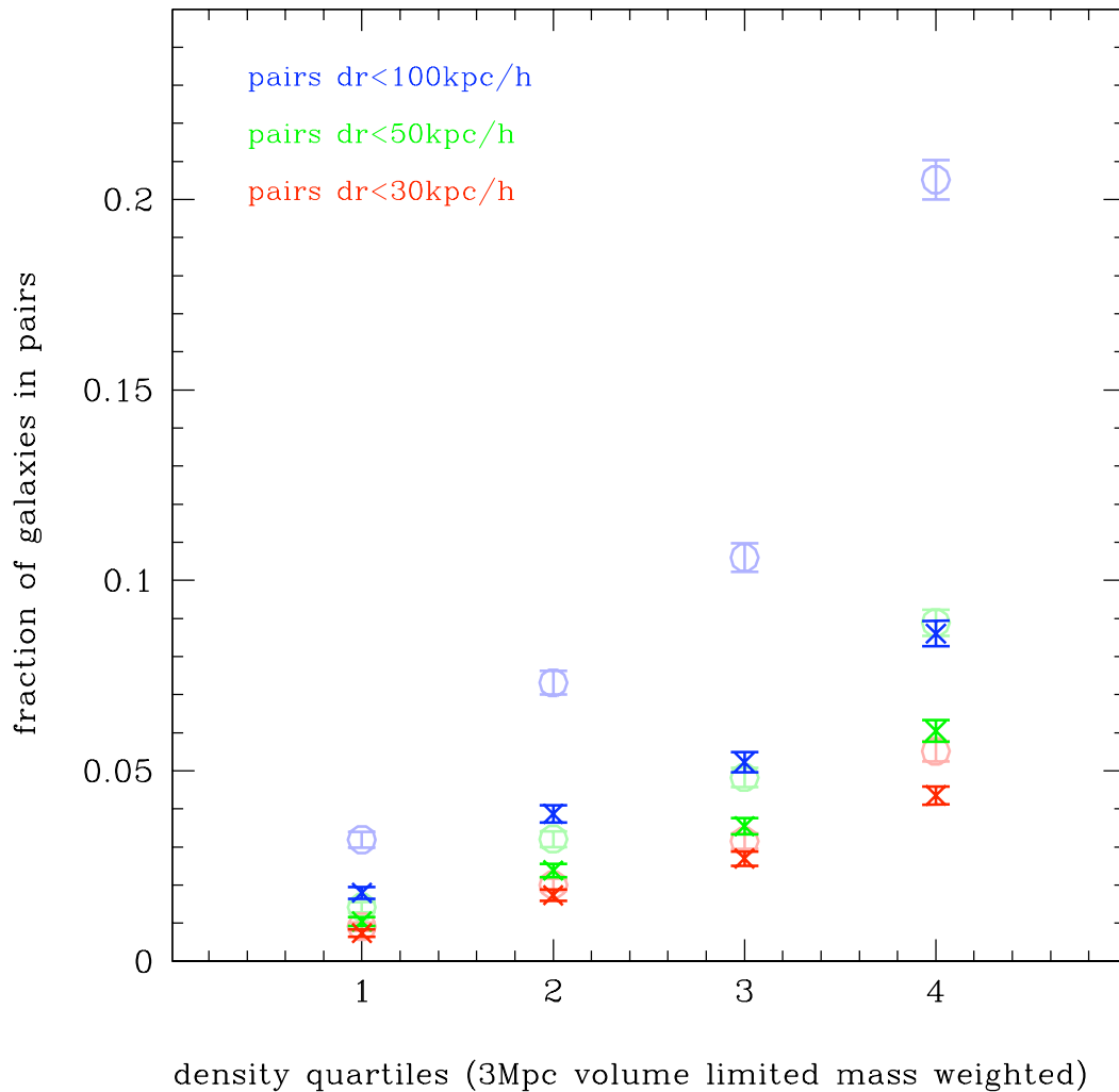
Fig. 8: The fraction of galaxies in the close kinematic pair systems in the Kitzbichler2006abcdef Millennium mocks in the redshift range 0.6 < z < 0.8 as a function of environment: over-densities are calculated as in our zCOSMOS sample. These are mass weighted, 3 Mpc constant-aperture with volume limited tracers: dr < 100 h^{-1}kpc in blue, dr < 50 h^{-1}kpc in green, and dr < 30 h^{-1}kpc in red, divided into quartiles of an underlying galaxy population. The “observed” fractions are indicated with open circles, while the crosses show the fractions of galaxies that are identified at 0.6 < z < 0.8 in pairs and which merged in the simulation by z = 0 .
