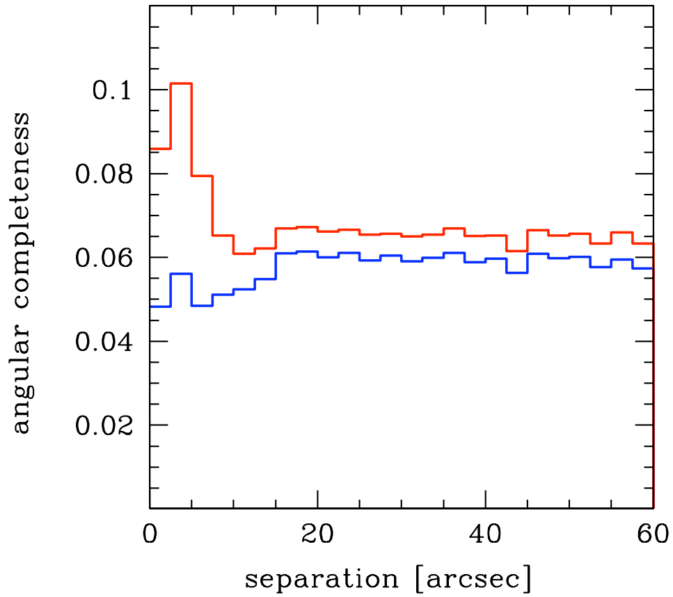
Fig. 2: The angular completeness of the 10k sample defined as the fraction of projected pairs in which both members were observed, compared with the case if all galaxies had been observed spectroscopically. Blue: only primary spectroscopic targets. Red: together with the secondary detections used in this analysis.
