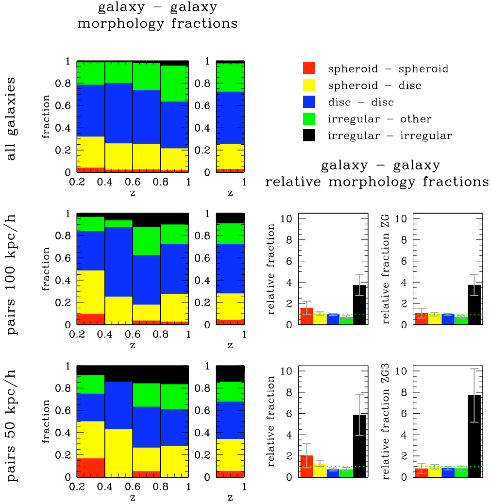
Fig. 12: Galaxy – galaxy morphological combinations of the close kinematic pair galaxies, color-coded according to the ZEST classification: black – type 3 & type 3 (irr – irr), green – type 3 & other, blue – type 2 & type 2 (disc-disc), yellow – type 1 & other, red – type 1 & type 1 (spheroid-spheroid). The top left panel presents galaxy – galaxy morphologies constructed from all of the possible pairs of all the galaxies in a given redshift bin regardless their distance. The narrow panel on the right shows an average galaxy – galaxy morphology fractions in the redshift range z=0.2-1 . With the same convention, the two mid-left panels present galaxy–galaxy morphological fractions for close kinematic pair galaxies with dr < 100 h^{-1}kpc , while the two bottom-left panels show close kinematic pair galaxies with dr < 50 h^{-1}kpc . The four panels on the right show the relative galaxy–galaxy morphological fractions of the close kinematic pair galaxies with a projected separations dr < 100 h^{-1}kpc & dr < 50 h^{-1}kpc in respect to the ones from the global sample and in respect to our preferred Monte Carlo models: ZG (for the pair sample with dr < 50 h^{-1}kpc ) and ZG3 (for the pair sample with dr < 100 h^{-1}kpc ).
