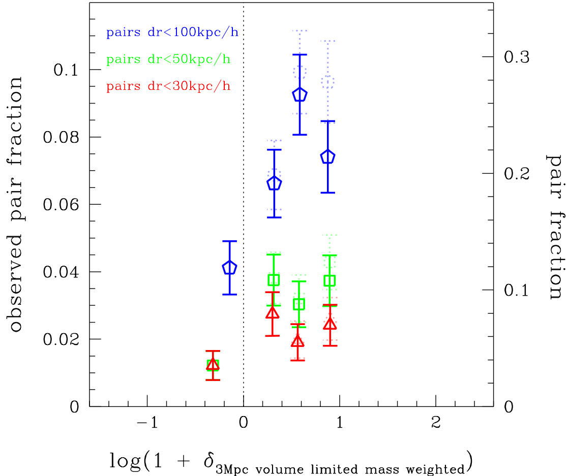
Fig. 5: The fraction of galaxies in close kinematic pair systems as a function of overdensity, computed as a mass-weighted, 3 Mpc constant aperture calculated with volume limited tracers, dr < 100 h^{-1}\text{kpc} in blue, dr < 50 h^{-1}\text{kpc} in green, and dr < 30 h^{-1}\text{kpc} in red, divided into quartiles of the density distribution of the underlying galaxy population. Dotted lines represent observed pair fractions, while the solid ones are after applying a correction for random unrelated projections as discussed Section 3.1. The left vertical axis shows the fractions observed in the 10k sample, the right axis shows the fractions expected in a complete, volume limited sample in which all galaxies were observed spectroscopically.
