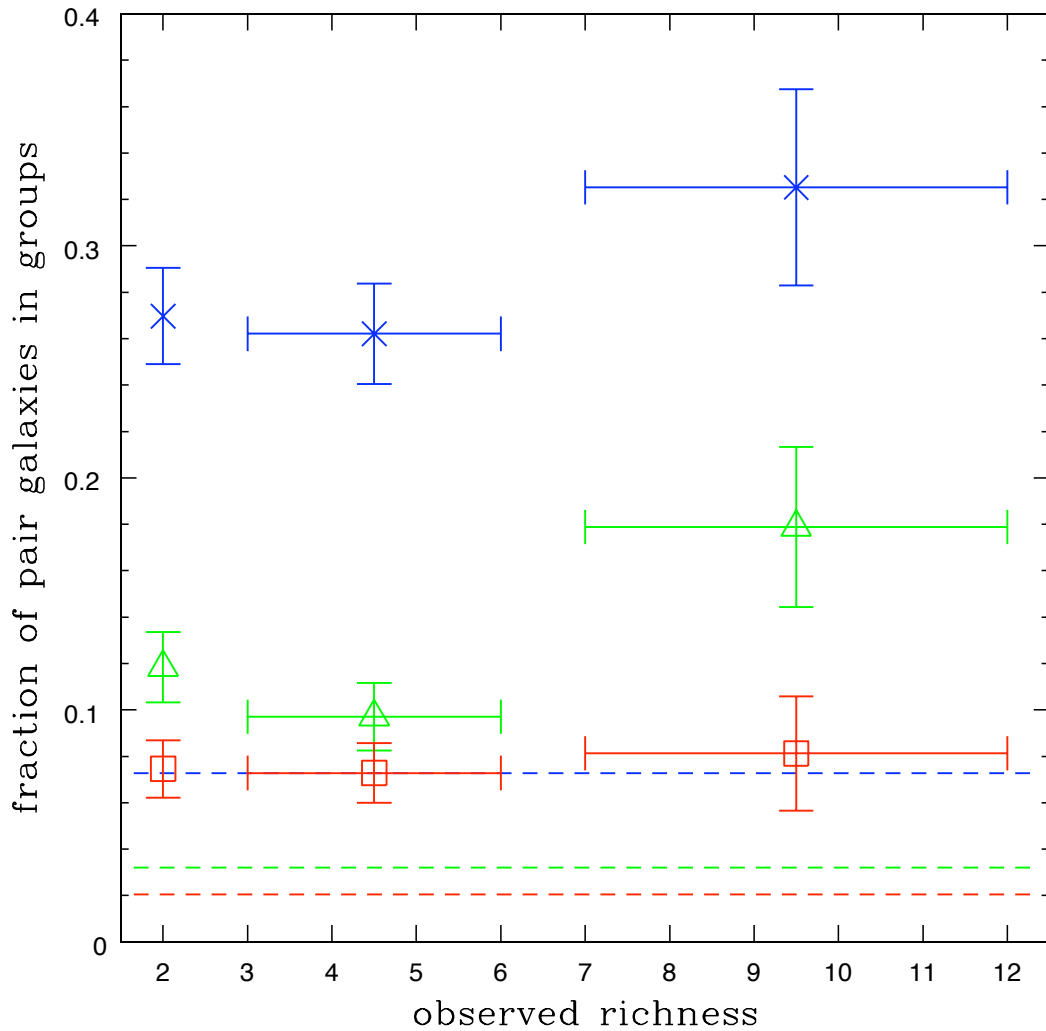
Fig. 9: The fraction of the galaxies in groups that are in the close kinematic pair systems at a given observed group richness, with dr less than 100 h^{-1}kpc (blue crosses), less than 50 h^{-1}kpc (green triangles), less than 30 h^{-1}kpc (red squares). Vertical error bars are the standard 1\sigma errors for the binomial distribution, while the horizontal ones show the binning. Dashed horizontal lines indicate the overall observed pair fraction calculated with respect to all of the galaxies in the volume limited zCOSMOS 10k sample, color-coded at the same projected distances.
