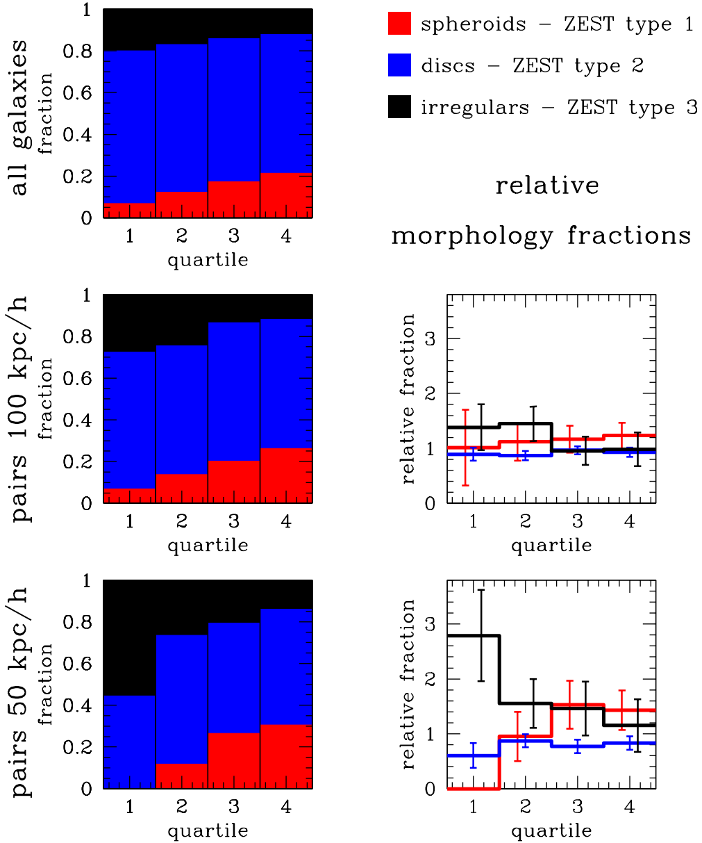
Fig. 15: Morphologies of the close kinematic pair galaxies as a function of overdensity quartiles. Top-left panel presents morphologies of all galaxies in an underlying sample in quartiles of the 3 Mpc constant aperture, mass weighted overdensities calculated with the volume limited tracers. Morphological types are color-coded according to the ZEST classification: red: type 1 (spheroid), blue: type 2 (disc), black: type 3 (irregular). With the same convention, the mid-left panel presents morphological fractions for the close kinematic pair galaxies with dr < 100 h^{-1} \text{kpc} , while the bottom-left one shows the close kinematic pair galaxies with dr < 50 h^{-1} \text{kpc} . Panels on the right show the relative morphological fractions of the close kinematic pair galaxies with a projected separations dr < 100 h^{-1} \text{kpc} (middle) and dr < 50 h^{-1} \text{kpc} (bottom) in respect to an underlying sample.
