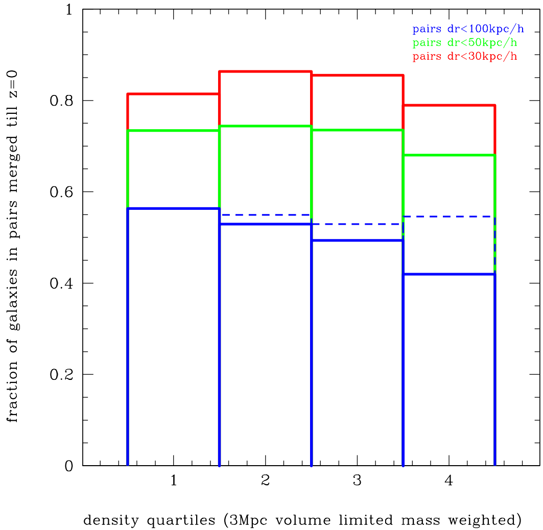
Fig. 7: The fraction of galaxies in pairs at 0.6 < z < 0.8 that merged in the Millennium simulation by z = 0 as a function of environment: dr < 100 h^{-1} \text{ kpc} in blue, dr < 50 h^{-1} \text{ kpc} in green, and dr < 30 h^{-1} \text{ kpc} in red. The dashed line indicates the fractions of galaxies in pairs with dr < 100 h^{-1} \text{ kpc} that would merge till z = 0 , after applying the correction for “spurious pairs” constructed in Section 3.1.
