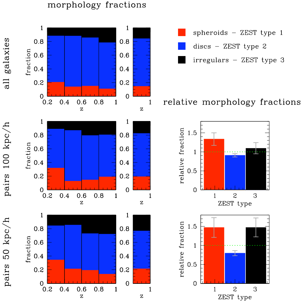
Fig. 10: Morphologies of the close kinematic pair galaxies. The top-left panel presents morphologies of all galaxies in the underlying sample (not matched in environment) in the different redshift bins. Different morphological types are color-coded according to the ZEST classification: red: type 1 (spheroid), blue: type 2 (disc), black: type 3 (irregular). Top right, the narrow panel shows the average morphological fraction through the redshift range z = 0.2 - 1 . With the same convention, the two mid – left panels show the morphological fractions for close kinematic pair galaxies with dr < 100 h^{-1}kpc , while the two bottom – left panels for close kinematic pair galaxies with dr < 50 h^{-1}kpc . Panels on the right show the relative morphological fractions of the close kinematic pair galaxies with a projected separations dr < 100 h^{-1}kpc & dr < 50 h^{-1}kpc in respect to the underlying sample.
