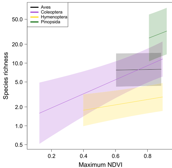
Figure 2. Responses of four taxa to changes in maximum NDVI. Aves (black line) showed no significant response to changes in maximum NDVI, while Coleoptera (purple line), Hymenoptera (yellow line) and Pinopsida (green line) showed a positive response to increasing maximum NDVI. Shaded areas indicate 95% confidence intervals.
