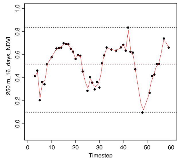
Figure 1. Time series of NDVI following a QualityScreen , as produced by an optional argument DiagnosticPlots in MODISSummaries , that illustrates the relationship between the three measures used: maximum time-series value, temporal mean, and temporal variability. On the y-axis is NDVI at 250 m 2 resolution (the axis label is the data band name for this Science Data Set). On the x-axis is time, with 16-day regular intervals. This time series produces a temporal variability value of 0.4. Variability is defined in the introduction of the main text. Upper black dashed line indicates the maximum value in the time series and the lower black dashed line indicates the minimum value in the time series. The solid red line indicates the interpolated values of the NDVI. Red dashed line indicates the mean of these values.
