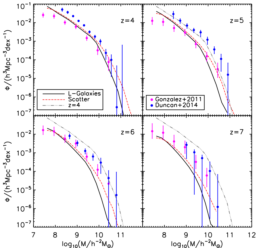
Figure 5. Predicted stellar mass functions at redshift z \approx 4 (top left), z \approx 5 (top right), z \approx 6 (lower left) and z \approx 7 (lower right). In each instance, we use the closest snapshot available to use from our L-GALAXIES run of z = 3.95, 5.03, 5.82 and 6.97 , respectively. Solid black lines show the stellar mass functions predicted by our model. To indicate the possible effect of uncertainties in the observational stellar mass determinations, we also show as a red dot-dashed line the stellar mass function convolved with a Gaussian of standard deviation 0.3 dex. Our z = 4 stellar mass function is repeated at higher redshifts as a grey dot-dashed line for comparison. Observations are taken from González et al. (2011), converted to a Chabrier IMF and Duncan et al. (2014).
