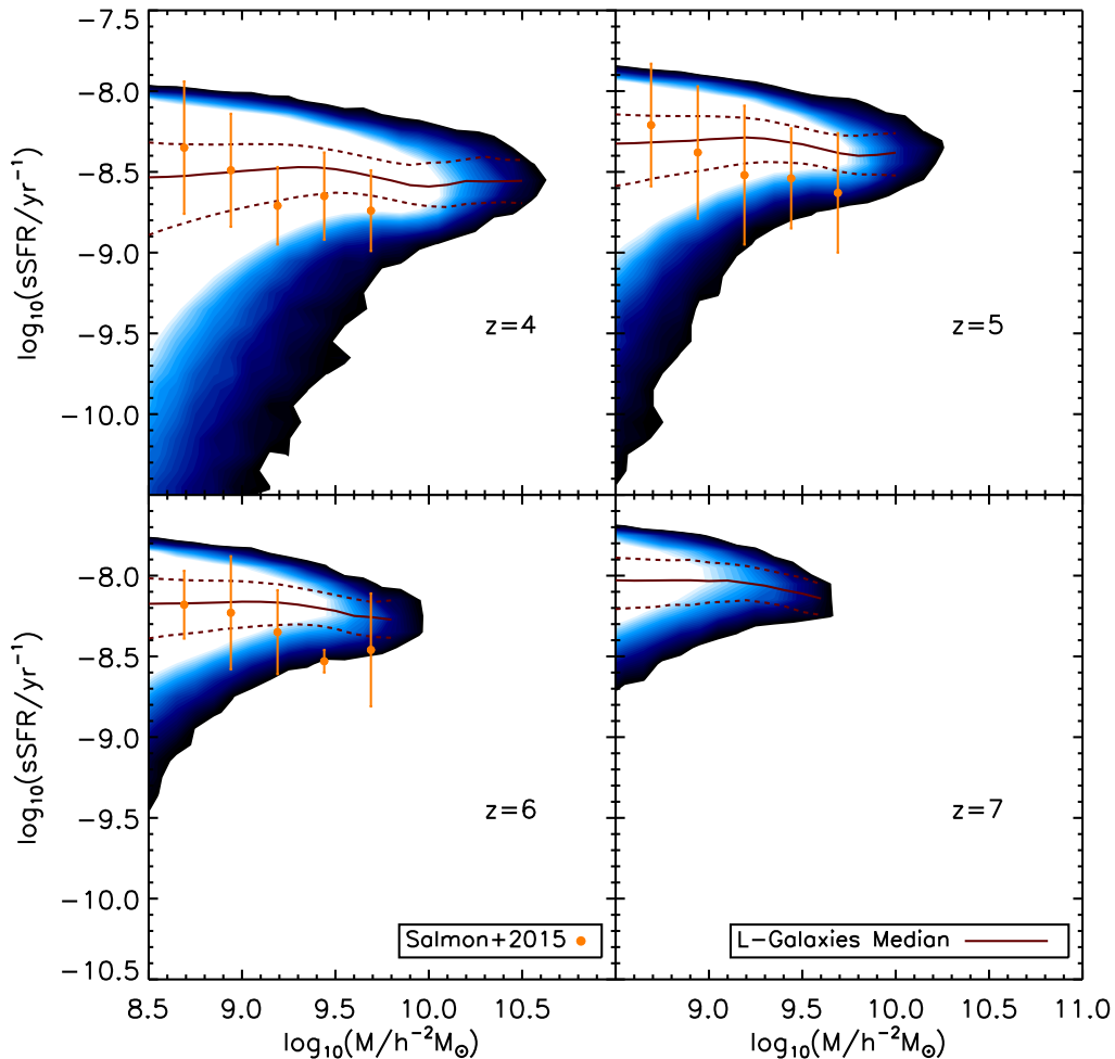
Figure 6. Predicted sSFRs ( \text{sSFR} = \text{SFR}/M ) at redshift z \approx 4 (top left), z \approx 5 (top right), z \approx 6 (lower left) and z \approx 7 (lower right). In each instance, we use the closest snapshot available to use from our L-GALAXIES run of z = 3.95, 5.03, 5.82 and 6.97 , respectively. The histogram density plot represents the L-GALAXIES galaxy population, with white representing the most dense, and blue representing the least. The solid line shows the L-GALAXIES median values, and the dashed lines show the 0.16 and 0.84 percentiles. The observations are taken from Salmon et al. (2015), the points denotes the median while the error bars reflect the scatter in the observed values (not the uncertainty on the median).
