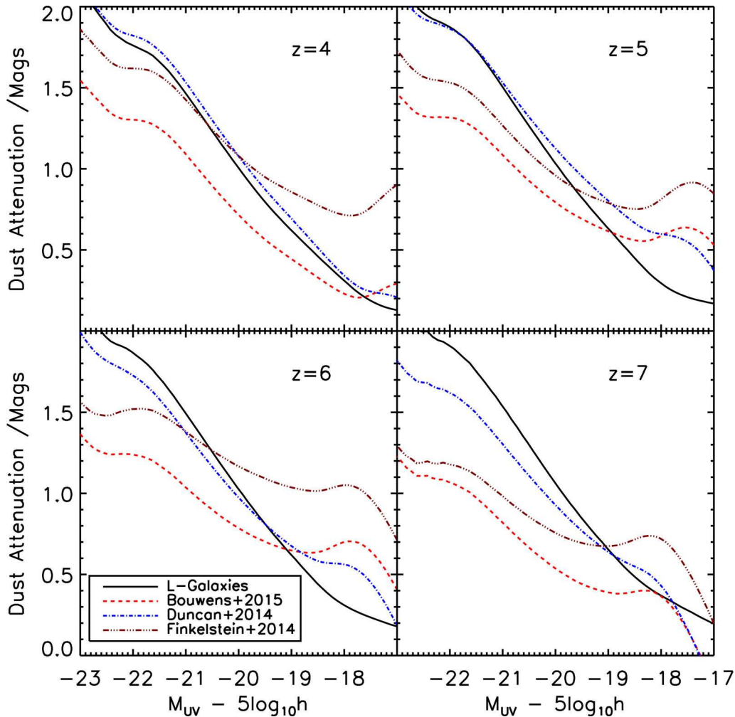
Figure 4. This figure shows the amount of dust attenuation required to move our intrinsic UVLF (the dashed, black lines in Fig. 3) to match different observational data sets (Duncan et al. 2014; Finkelstein et al. 2014; Bouwens et al. 2015), as a function of unattenuated absolute UV magnitude. The solid, black line shows the attenuation built into the L-GALAXIES model as described in Section 2.2.
