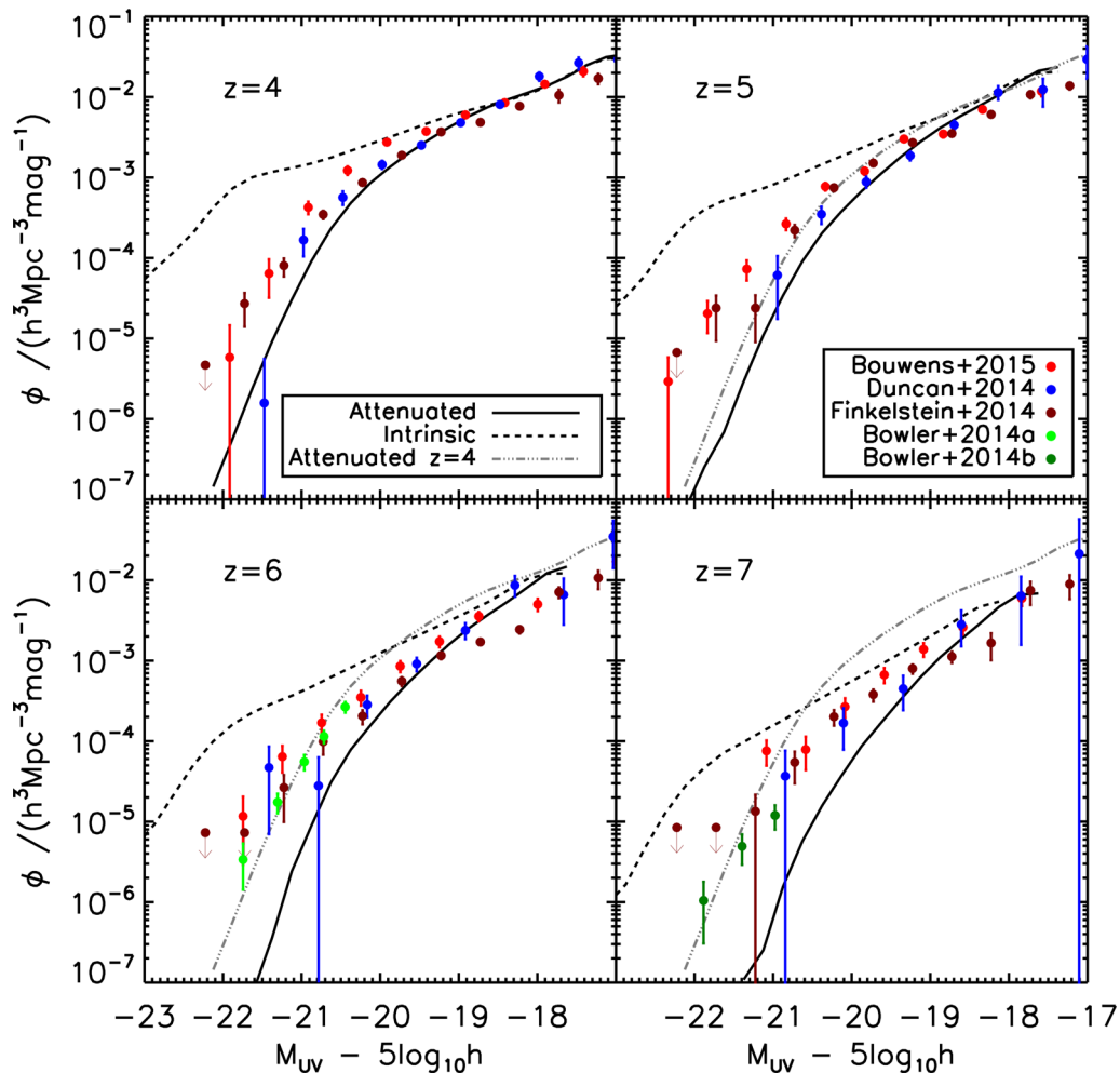
Figure 3. Predicted rest-frame (1500 Å) UVLF at redshift z \approx 4 (top left), z \approx 5 (top right), z \approx 6 (lower left) and z \approx 7 (lower right). In each instance, we use the closest snapshot available to use from our L-GALAXIES run of z = 3.95, 5.03, 5.82 and 6.97 , respectively. Solid black lines shows the L-GALAXIES prediction for the attenuated UVLF using the dust extinction model outlined in Section 2.2.1. The dashed black line is the L-GALAXIES prediction of the intrinsic UVLF, with no dust model applied. Our z = 4 attenuated, UVLF is repeated at higher redshifts as a grey dot-dashed line for comparison. Observations are taken from Bouwens et al. (2015), Duncan et al. (2014) and Finkelstein et al. (2014); and at high mass from Bowler et al. (2014a, z = 6 ) and Bowler et al. (2014b, z = 7 ).
