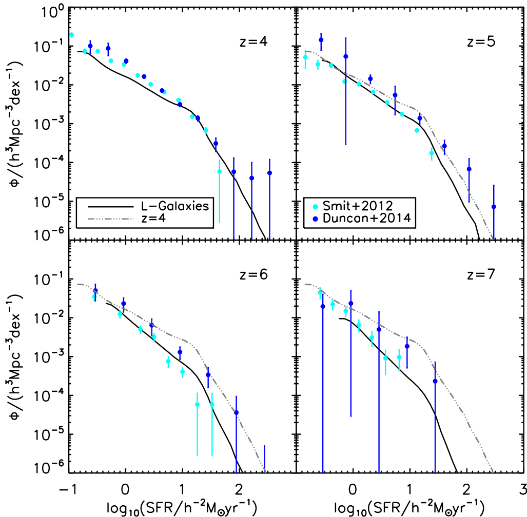
Figure 2. Predicted SFRDF at redshift z \approx 4 (top left), z \approx 5 (top right), z \approx 6 (lower left) and z \approx 7 (lower right). In each instance, we use the closest available snapshot from our L-GALAXIES run of z = 3.95, 5.03, 5.82 and 6.97 , respectively. Solid black lines show the SFRDF predicted by our model. Our z = 4 SFRDF is repeated at higher redshifts as a grey dot-dashed line for comparison. Observations are taken from Smit et al. (2012), converted to a Chabrier IMF, and Duncan et al. (2014).
