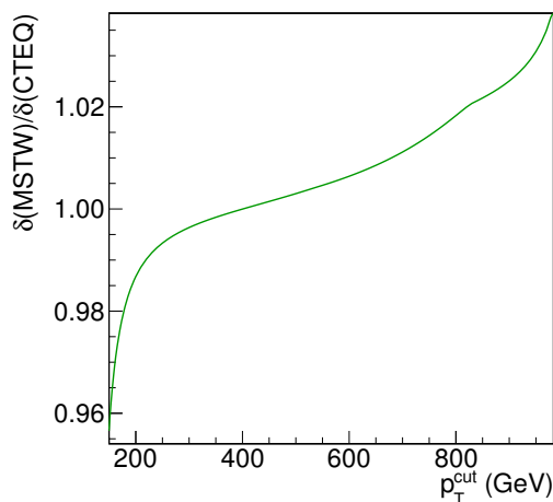
Figure 7. The ratio of \delta(p_T^{\text{cut}}) calculated with MSTW2008n1o68c1 parton distribution functions to \delta(p_T^{\text{cut}}) calculated with cteq6mE. The top-partner used for calculating \delta(p_T^{\text{cut}}) has mass 1 TeV and mixing angle \sin^2(\theta_R) = 0.4 . All distributions were generated using 8 TeV LHC parameters.
