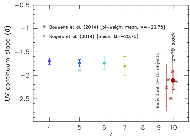
Figure 4. The observed UV-continuum slope as a function of redshift for candidate high-redshift ( z = 4\text{--}10 ) star-forming galaxies. Results at z = 4\text{--}7 are based on the bi-weight mean of galaxies with M_{1500} \approx -20.75 from Bouwens et al. (2014a).
