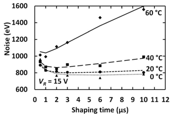
FIG. 13. Total measured (60°C—diamonds; 40°C—squares; 20°C—circles; 0°C—triangles) and calculated (60°C—solid line; 40°C—long dashes; 20°C—square dots; 0°C—round dots) FWHM of 5.9 keV peak as a function of shaping time at 15 V reverse bias.
