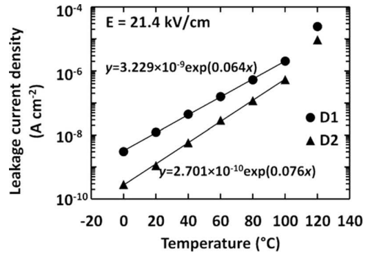
FIG. 4. Measured leakage current density as a function of temperature at 21.4 kV/cm internal electric field for D1 (circles) and D2 (triangles). The line of best fit at the temperature range 0°C to 100°C can also be seen.
