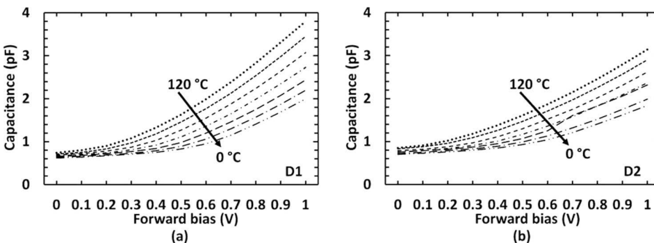
FIG. 6. Capacitance as a function of applied forward bias for (a) D1 and (b) D2 in the temperature range 0^\circ\text{C} to 120^\circ\text{C} .
