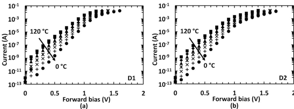
FIG. 1. Current as a function of applied forward bias for (a) D1 and (b) D2 in the temperature range 0 °C to 120 °C.
