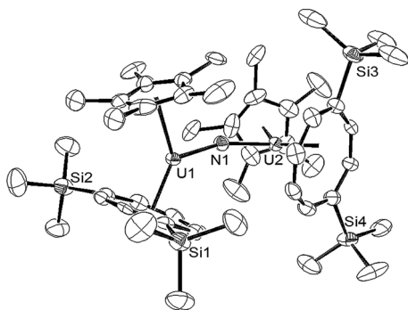
Fig. 4 ORTEP-3 diagram of the molecular structure of the anion in (10) displaying 50% probability ellipsoids. H atoms have been removed for clarity. Selected bond-lengths (Å) and angles (°): N1–U1 2.063(5), U2–N1 2.066(5), Ct(COT)–U1 2.033(4), Ct(Cp*)–U1 2.516(2), Ct(COT)–U2 2.038(4), Ct(Cp*)–U2 2.536(2); U1–N1–U2 159.4(3), Ct(COT)–U1–Ct(Cp*) 137.03(2), Ct(COT)–U2–Ct(Cp*) 136.70(2), Ct(COT)–U1–N1 122.83(8), Ct(Cp*)–U1–N1 100.09(1), Ct(COT)–U2–N1 122.75(3), Ct(Cp*)–U2–N1 100.54(2).
