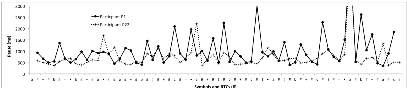
Fig 5. Pauses for symbol and RTC actions (#,•) by the least (P1) and most (P22) competent participants.
