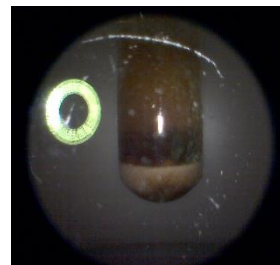
Figure 4. Flocculation of the potassium phosphate, demonstrating that no stirring occurs in the microwave vessel while the solvent is boiling.
