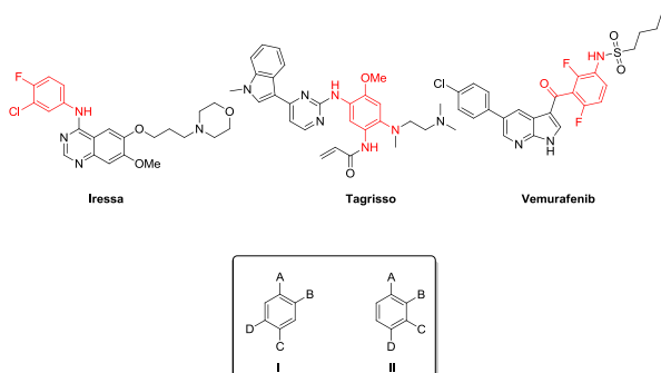
Figure 1. Examples of 1,2,4,5- and 1,2,3,4- substituted aromatic scaffolds.
