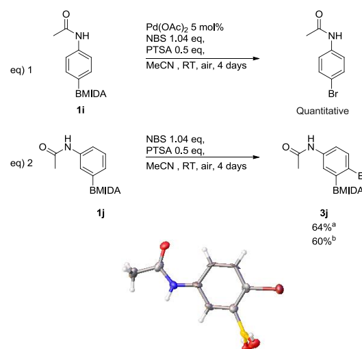
Scheme 5. Attempted bromination via ortho -selective C-H activation, including x-ray structure of 3j' (MIDA protection was cleaved in crystallisation process). a with 5 mol% Pd(OAc) 2 , b without Pd(OAc) 2 .
