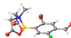
Figure 3. Solid state structure of 3b .
