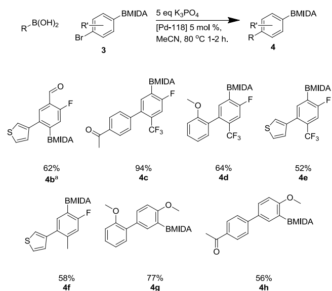
Scheme 8. Aqueous deprotection Suzuki cross-couplings.
