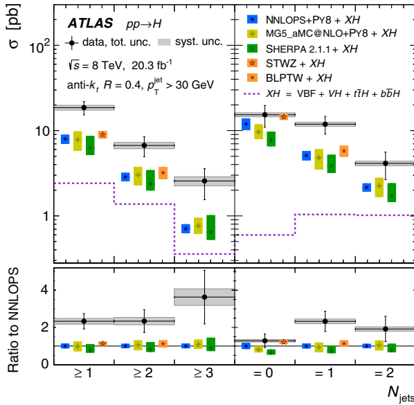
FIG. 2 (color online). Measured Higgs boson production cross sections in inclusive and exclusive jet multiplicity bins compared to different theoretical predictions (see Table I for details and references).
