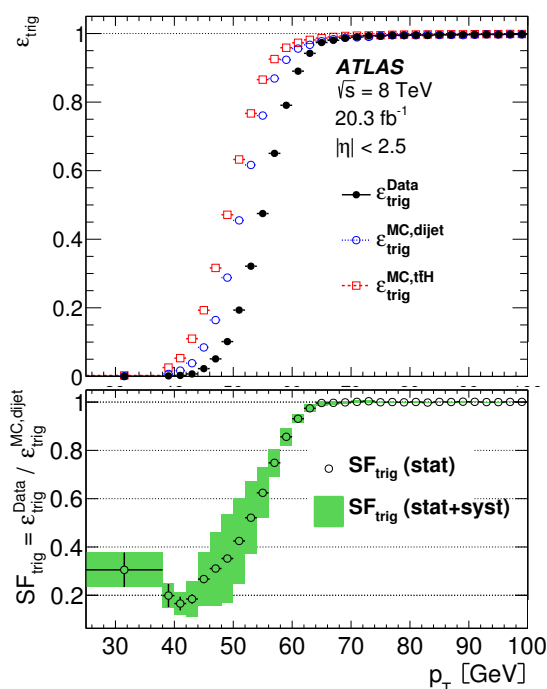
Figure 4. Single-jet trigger efficiencies, \epsilon_{\text{trig}} , (top) for data, simulated dijet events, and t\bar{t}H events, as a function of jet p_T for jets with |\eta| < 2.5 ; (bottom) SF_{\text{trig}}(p_T, \eta) = \epsilon_{\text{trig}}^{\text{data}}(p_T, \eta) / \epsilon_{\text{trig}}^{\text{MC,dijet}}(p_T, \eta) . The uncertainty on SF_{\text{trig}} , shown as the green shaded area, is estimated from the difference between the efficiencies in dijet and t\bar{t}H simulated events in the denominator of SF_{\text{trig}} .
