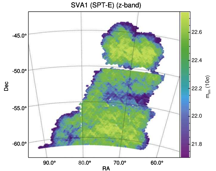
Figure 1. Map of 10\sigma depth (in magnitudes) in \sim 125 deg 2 in the SVA1 SPT-E footprint for SLR-corrected z_{\text{auto}} magnitudes. Small-scale variations are caused by variations in the number of exposures, chip gaps, and observing conditions.
