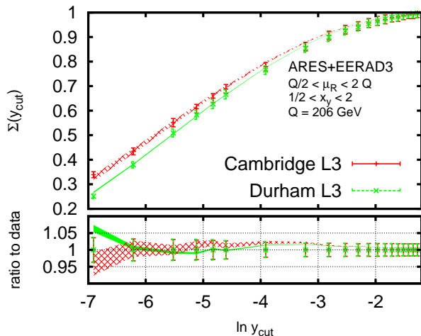
FIG. 2: Comparison of NNLL+NNLO predictions for the two-jet rates to data from the L3 collaboration [27].
