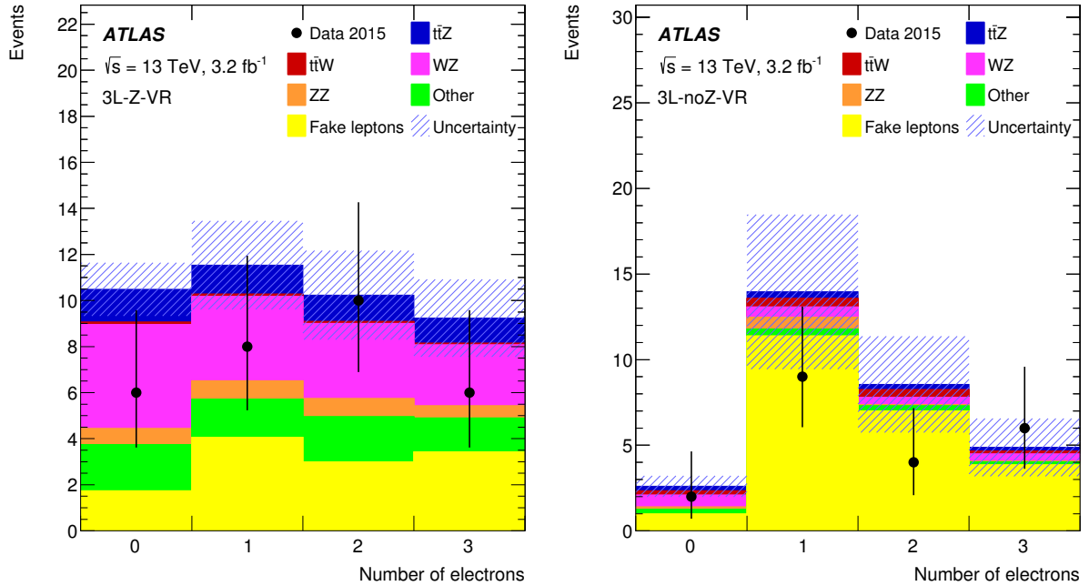
Figure 3: Distributions of the number of electrons in the (left) 3\ell -Z-VR and (right) 3\ell -noZ-VR validation regions, shown before the fit. The background denoted ‘Other’ contains other SM processes producing three prompt leptons. The shaded bands include statistical and systematic uncertainties in the SM prediction.
