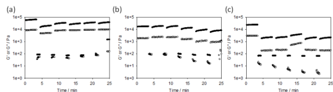
Figure 3. Recovery tests for (a) Ca-triggered gels; (b) acid-triggered gels; (c) Solvent-triggered gels. In all cases, the gels were subjected to a constant frequency of 10 rad/s and strain of 0.5% for 200 seconds, followed by a higher strain of 500% for 60 seconds. Restoration of the gel was monitored in the subsequent time sweep (again at a frequency of 10 rad/s and strain of 0.5%). These cycles were repeated five times. The data at 300% and 1000% strain are shown in the Supporting Information.
