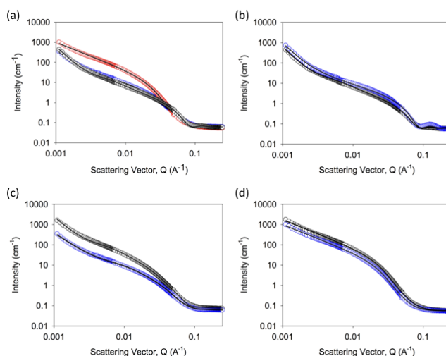
Figure 4. SANS data for gels formed from 2NapFF. (a) Overlay of data for gels formed at a concentration of 5 mg/mL (black data shows data for Ca-triggered gels; blue data are for acid-triggered gels, and red data for solvent-triggered gels; (b) Data for Ca-triggered gels; (c) Data for acid-triggered gels; (d) Data for solvent-triggered gels; For (b) – (d), the data at 5 mg/mL are shown in blue and the data at 10 mg/mL are shown in black. In all cases, the fits to the data are shown as the line through the open symbols.
