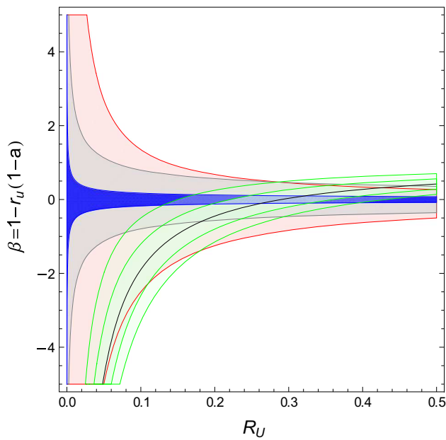
Fig. 2 Allowed parameter space for the vector-singlet U from \Delta B_s = 2 (blue region), R_{D^{τ/l}} (green), R_{K^{(*)ν}} (red) and \mathcal{B}(K^+ \rightarrow \pi^+ \nu \bar{\nu}) (gray). R_U = 4g_U^2 M_W^2 / g^2 M_U^2
