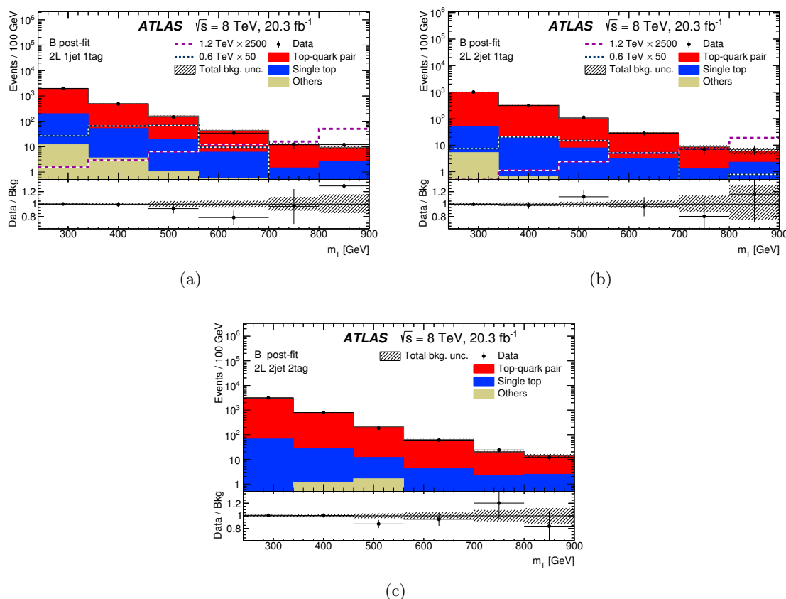
Figure 10. Distributions of the discriminant variable, transverse mass, m_T , in the dilepton channel for data and SM background processes in the (a) 2L\ 1jet\ 1tag signal region, (b) 2L\ 2jet\ 1tag signal region and (c) 2L\ 2jet\ 2tag control region using the B selection. The two B signal distributions that are included for the signal region distributions are scaled to the theory cross-sections multiplied by the indicated factor for better visibility. The background processes are normalised to their post-fit normalisation. The uncertainty band includes statistical and all systematic uncertainties. The first and the last bin contain the underflow and overflow, respectively. The binning of the figures is the same as used in the binned likelihood fit function.
