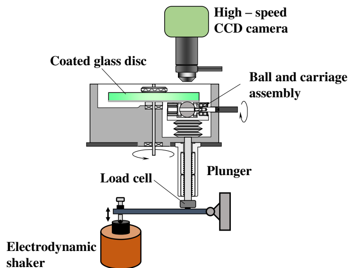
Figure 2. Experimental setup.
