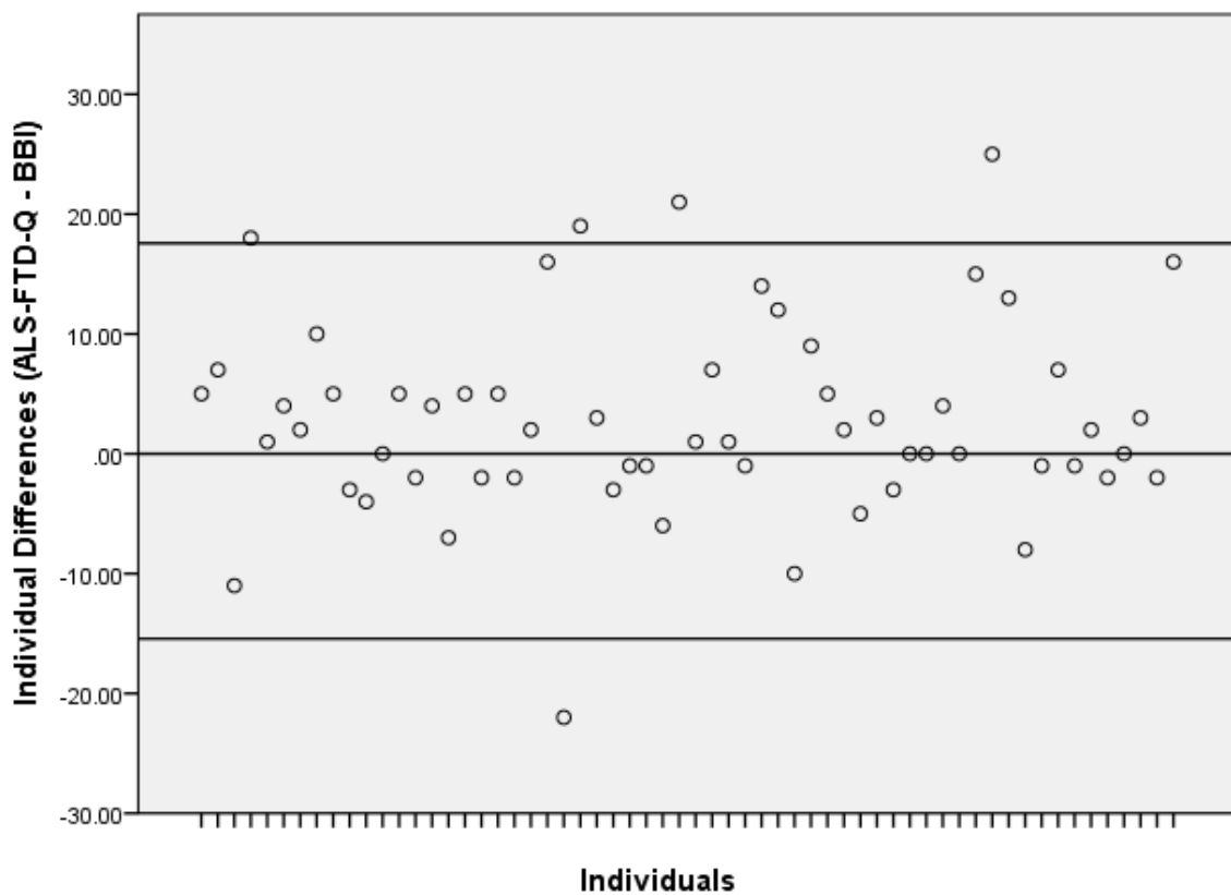
Figure 1. Bland-Altman Plot of within individual's measurements differences
