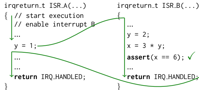
Fig. 2: Motivating example
