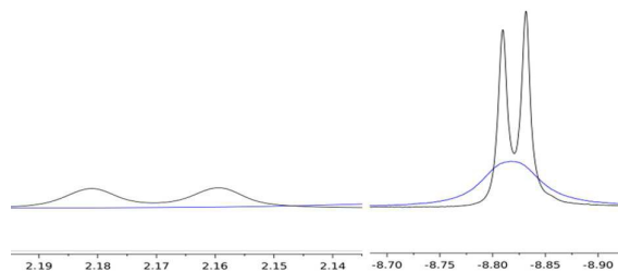
Figure 2: Hydride peaks in ( 4 ) at RT (blue) and at 0 °C (black).
