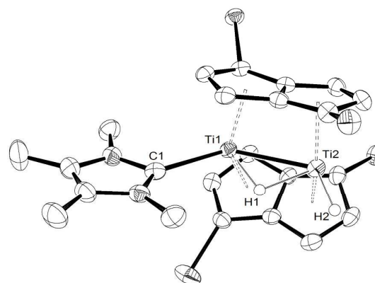
Figure 3: ORTEP diagram of the molecular structure of ( 4 ) displaying 50% probability ellipsoids. i Pr groups omitted for clarity.
