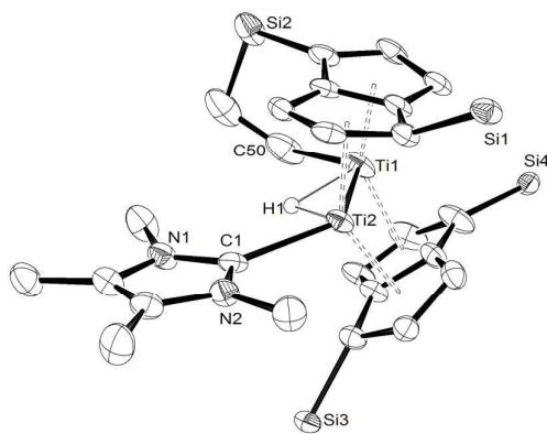
Figure 1: ORTEP diagram of the molecular structure of ( 3 ) displaying 50% probability ellipsoids. i Pr groups omitted for clarity
