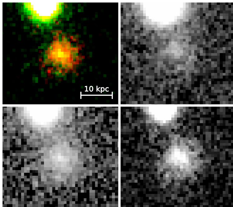
Fig. 2. The 4.2'' \times 3.7'' regions centered on HAE229. Top left panel: A composite three-color image made by combining the Y-, H-, and K-band color images taken with HAWK-I on the ESO/VLT (see text and Table 2 for details). To show the rest-frame blue and red optical morphology, we show each color component of the composite separately, namely, Y-band (approximately rest-frame U-band, top right), H-band (approximately rest-frame B- or V-band, bottom left) and K_s -band (approximately rest-frame R-band, bottom right). The Y-band image has a morphology similar to that of the F814W image and no offset is detected between the rest-frame UV and rest-frame optical regions. With increasing wavelength, the emission becomes less clumpy, more regular, and a red nucleus is evident. The dynamical center of the CO(1-0) emission corresponds to the highest surface brightness region of the H- and K_s -band images suggesting this region is also the center of mass of the galaxy. The bright galaxy above HAE229 in all panels lies at z_{phot} \approx 0.5 (Tanaka et al. 2010).
