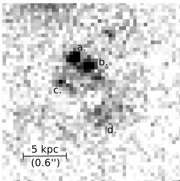
Fig. 1. The 3'' \times 3'' HST F814W image of the clumpy galaxy, HAE229. The size of HAE229 is 1''.2 \times 0''.6 ( 10 \times 5 kpc). Regions a and b are clumpy and knot-like whereas areas c and d have more diffuse rest-frame UV emission morphology.
