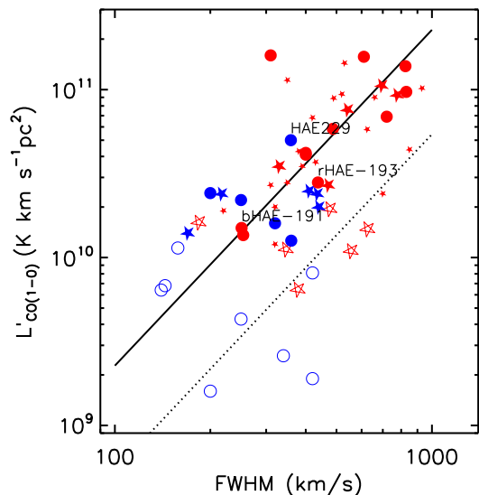
Fig. 7. Relation between FWHM of the CO(1-0) line and L'_{\text{CO}} for cluster (circles) and field galaxies (stars). High-redshift sources, those with z > 1 , are indicated by filled symbols while sources with z < 1 are indicated by hollow ones. The color-coding used in the figure is as follows: intermediate- z ULIRGs (red hollow stars Magdis et al. 2014), normal SFGs at z = 1.5 (blue filled stars Daddi et al. 2010a; Aravena et al. 2014), and SMGs (large and small red filled stars from Ivison et al. 2011; Bothwell et al. 2013, respectively). References for cluster sources can be found in section 5.2 and Table A.1. The mode of star formation for each source is color-coded as blue for “disk-like” and red for “starburst”. The solid line shows the relation from Bothwell et al. (2013). The dashed line assumes the typical radius for disk galaxies. Both high- z population, dusty starbursts, and disk-like galaxies show a unique correlation between CO luminosity and line width with significant scatter ( \sim 0.3 dex).
