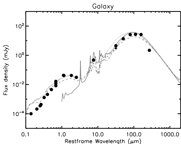
Fig. 5. Spectral energy distribution of HAE229 (black filled circles). We show the template SED (solid line) of a main-sequence galaxy at z = 2 (Magdis et al. 2012) which is based on models (Draine & Li 2007). In addition, template SEDs of observed SMGs are shown for comparison: ALESS SMG composite (dotted line Swinbank et al. 2014), average SED of 73 spectroscopically identified SMGs (dashed line Michałowski et al. 2010), and an average SED of SMGs (dashed-dotted line Pope et al. 2008). The far-infrared SED is matched by the different SMG composites whereas the rest-frame optical SED shows that HAE229 is redder than the average of various types of dusty vigorously star-forming galaxies at high redshift.
