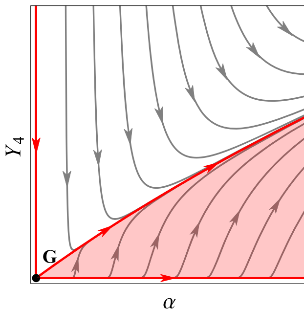
Fig. 2 Phase diagram of gauge–Yukawa theories with B > 0 and C < 0 at weak coupling showing asymptotic freedom and the Gaussian UV fixed point ( G ). Arrows indicate the flow towards the IR. The red-shaded area covers the set of UV complete trajectories emanating from the Gaussian UV fixed point. The Yukawa nullcline acts on trajectories as an IR attractor
