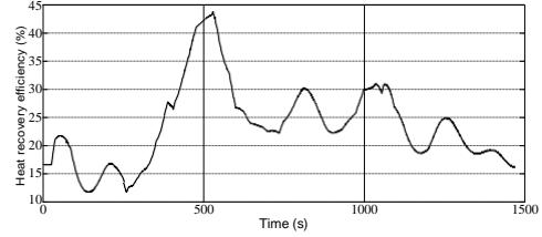
Figure 16. Heat recovery efficiency
