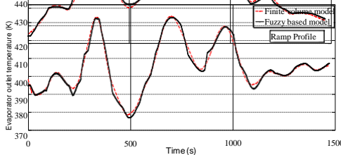
Figure 9. Prediction of the evaporator outlet temperature with respect to ramp profile.
