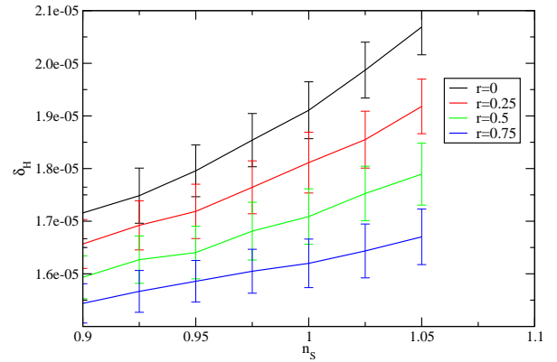
FIG. 1: The WMAP3 normalization \delta_{\text{H}} as a function of n for the four choices of r , specified at the scale 0.05 \text{ Mpc}^{-1} . The uncertainties shown are the standard deviations inferred from the Markov chains.
