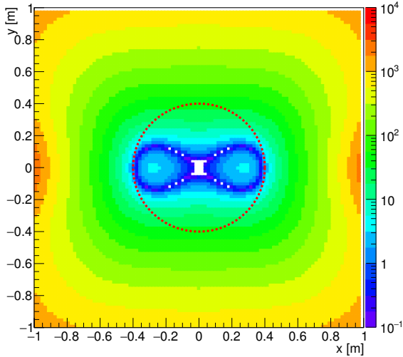
(a) B_0 uniformity in the XY plane in pT.
