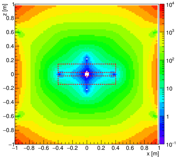
(b) B_0 uniformity in the XZ plane in pT.
